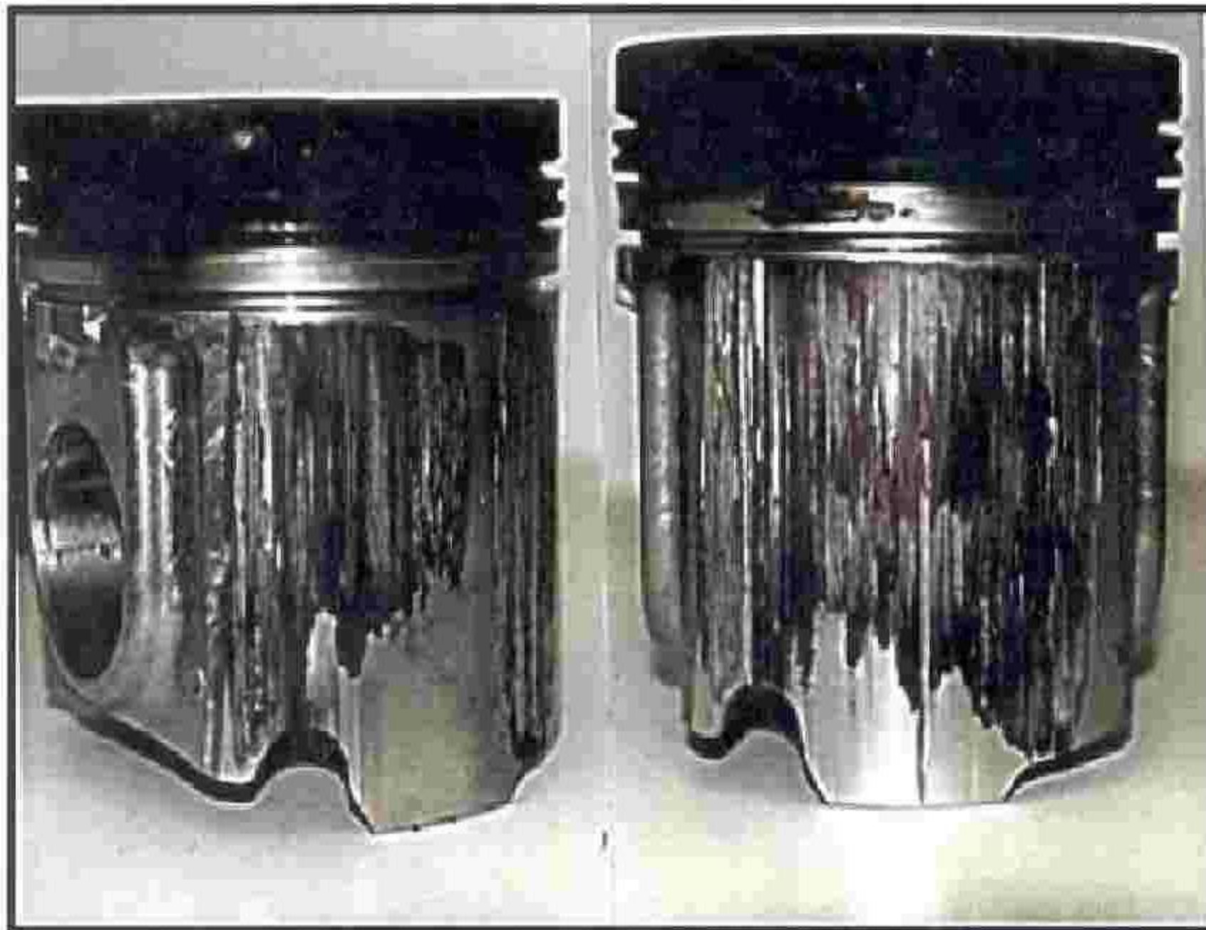
1-K CATERPILLAR TEST PISTON (Outer Surfaces of a Different Piston using another additive Not Sustaining the 1-K Test Conditions)
